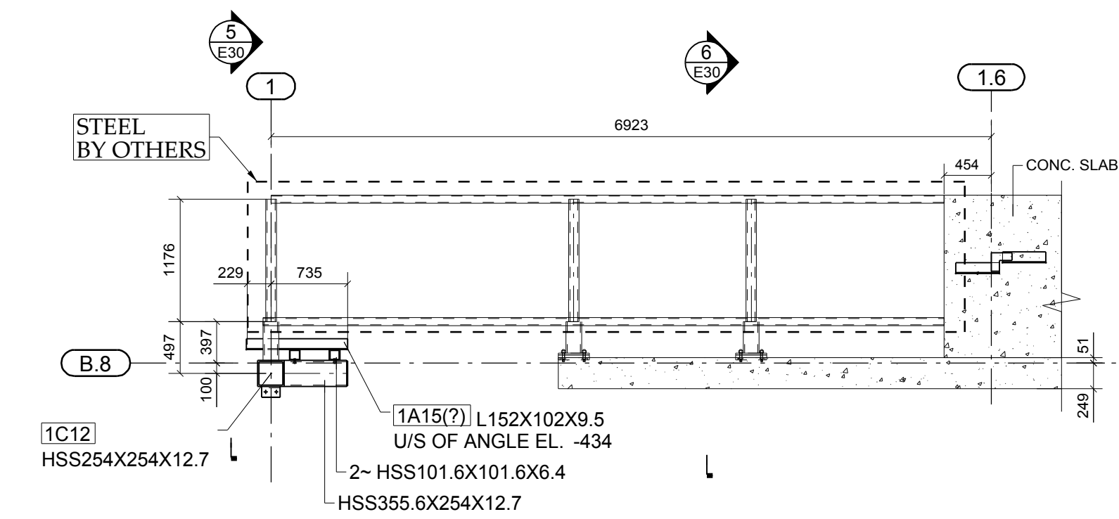
PARTIAL GROUND FLOOR PLAN - SECTOR 2 REF.SHEET.S2.02B
