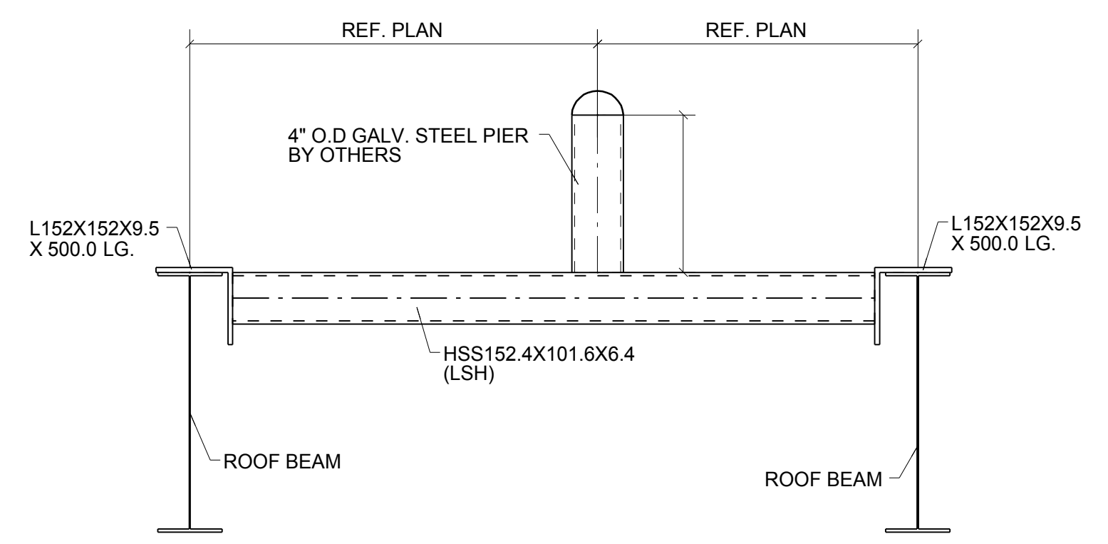
TYPICAL ROOF ANCHOR CONNECTION DETAIL
