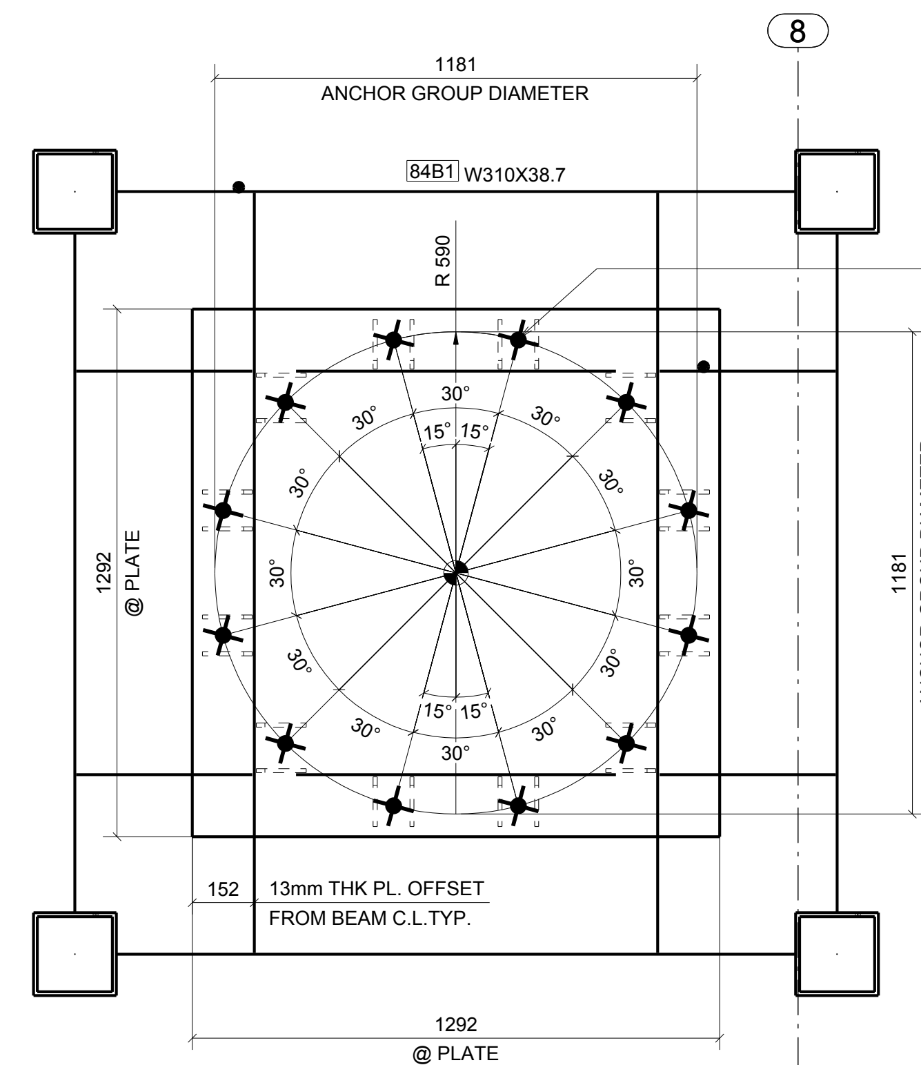
DETAILED VIEW FOR ANCHOR ROD LOCATION
