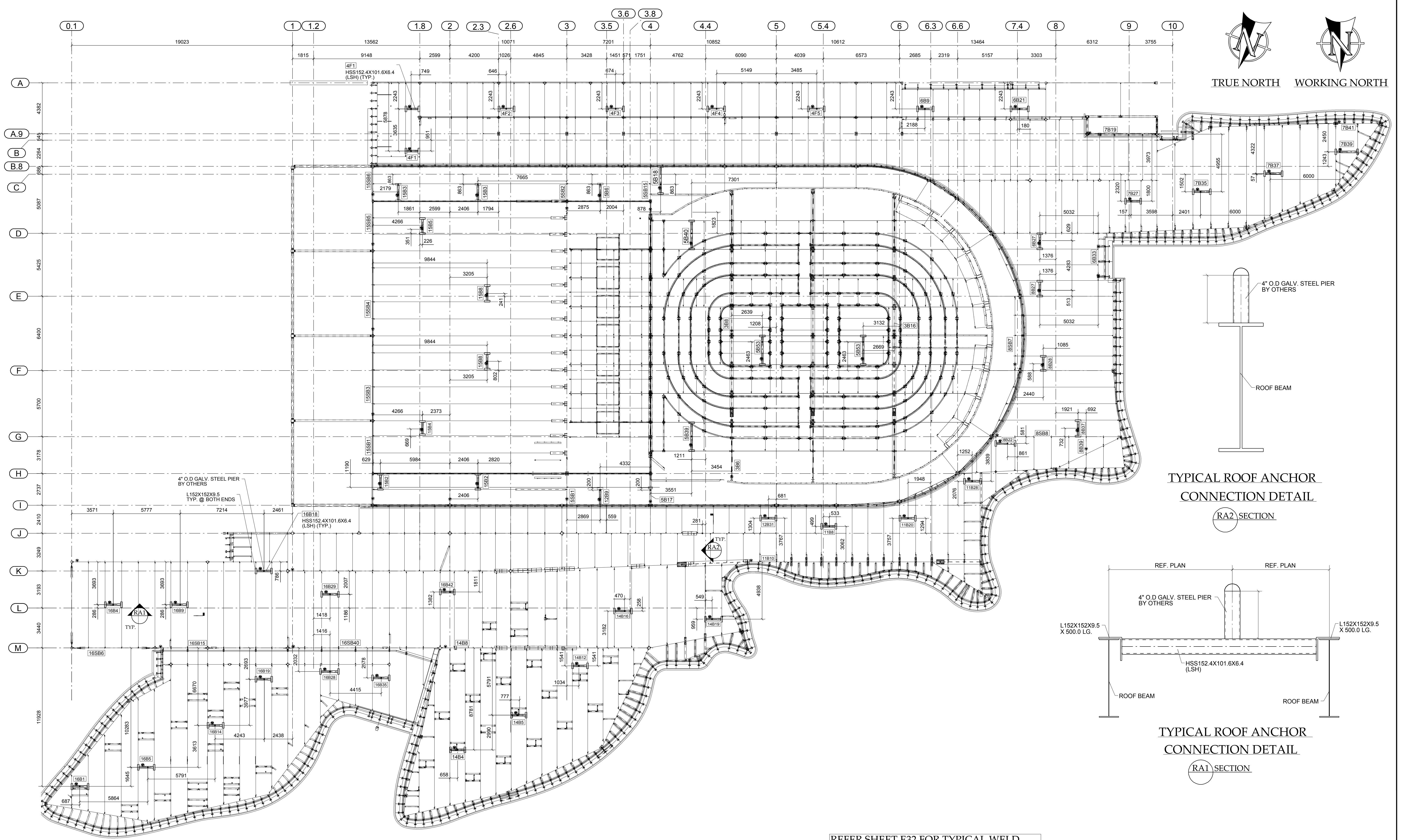
ROOF ANCHOR LAYOUT
