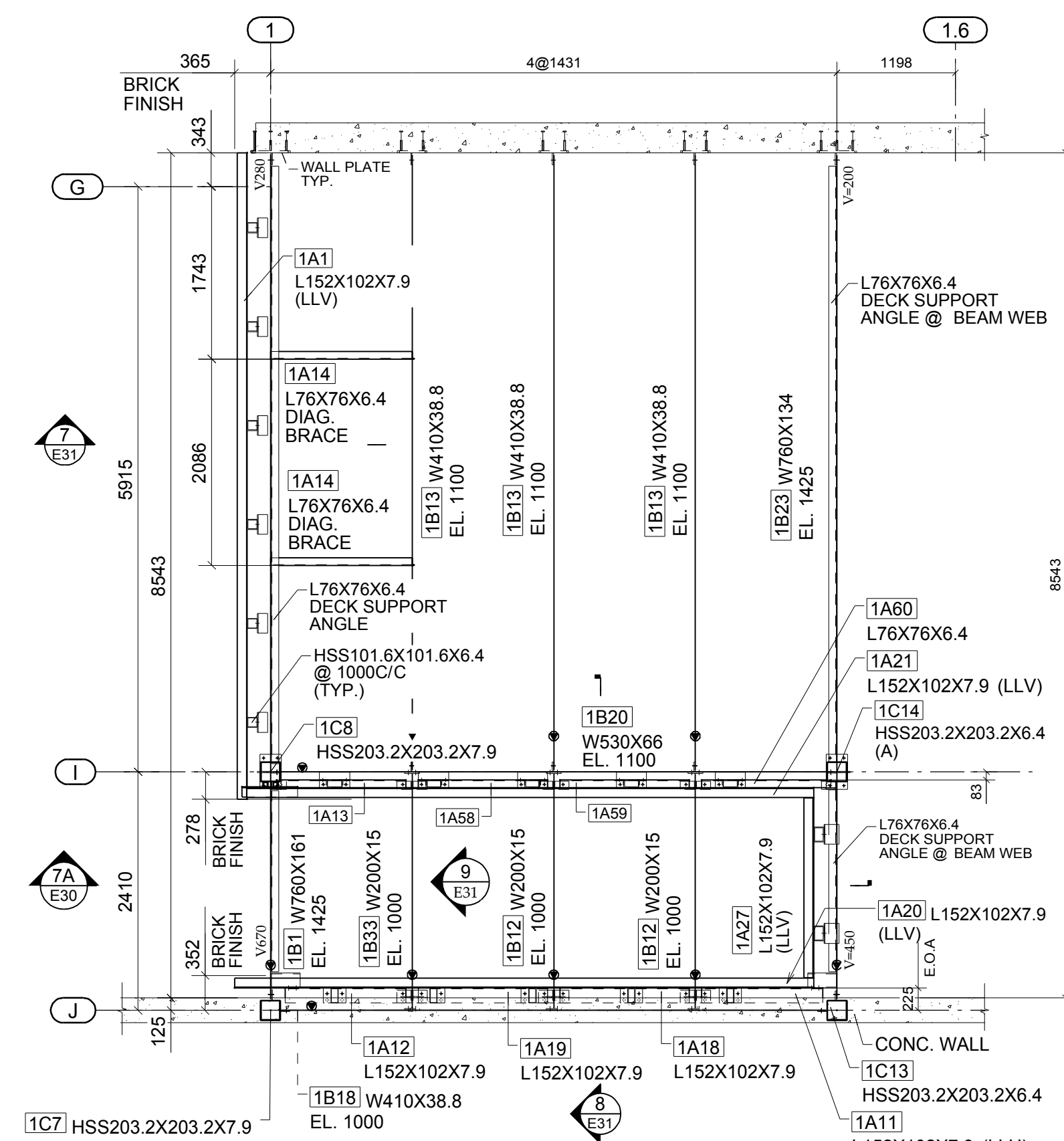
PARTIAL GROUND FLOOR PLAN - SECTOR 1 REF.SHEET.S2.02A
